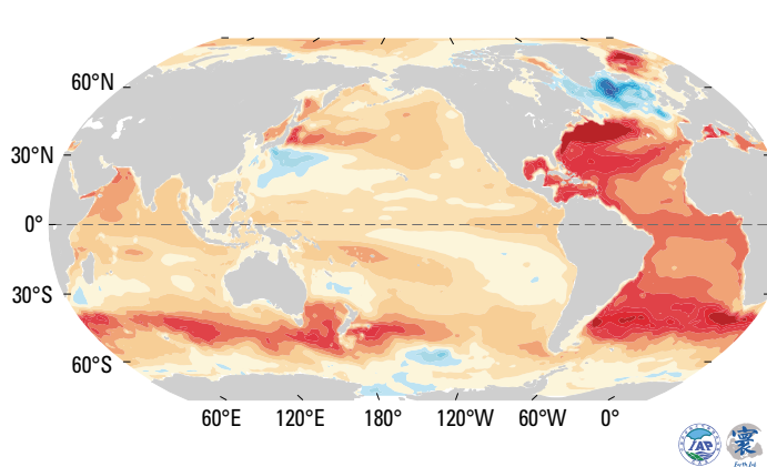
Figure 5. Observed upper 2000 m OHC trend from 1958 to 2023.
